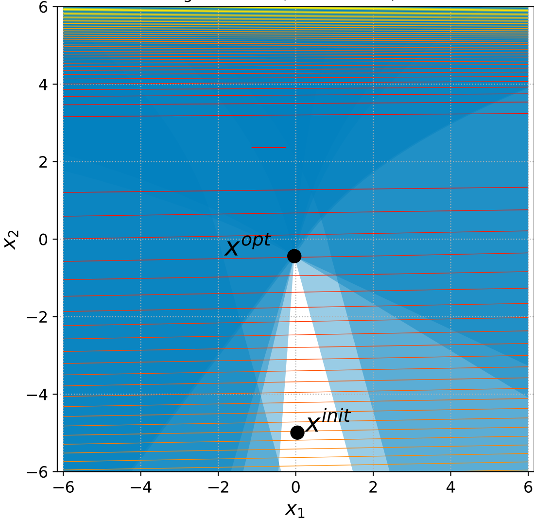
34 Bent Cigar with 6+n/2 constraints, instance=4
