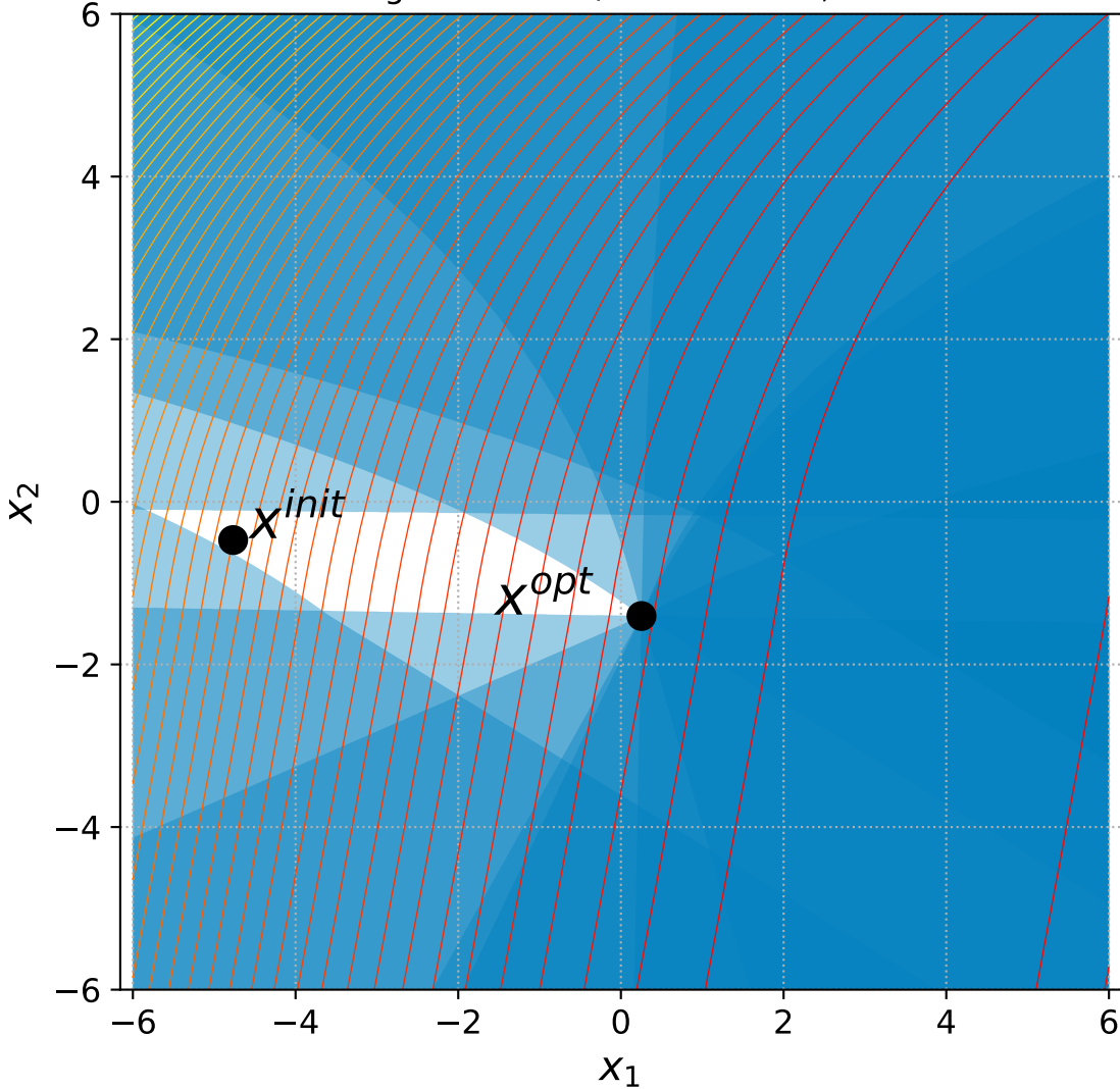
34 Bent Cigar with 6+n/2 constraints, instance=3
