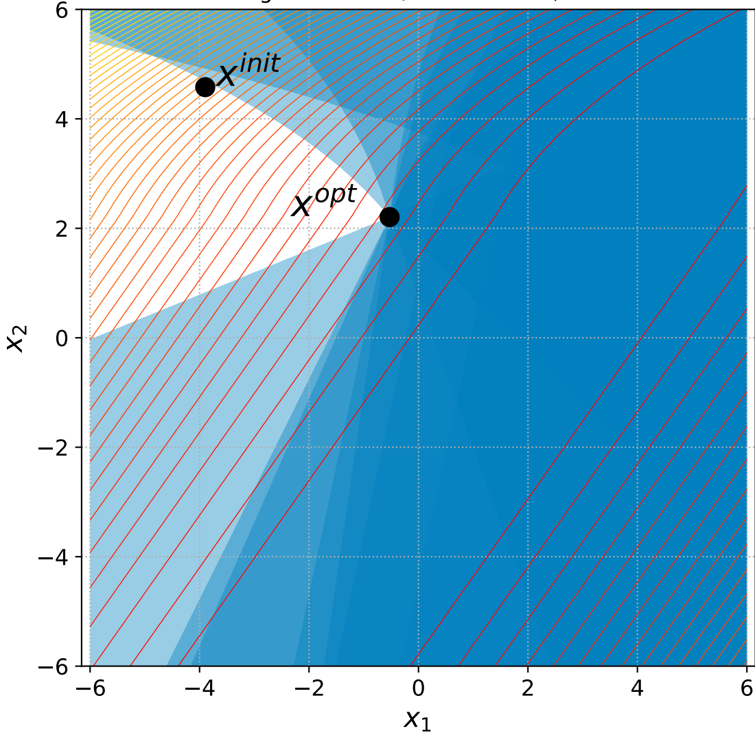
34 Bent Cigar with 6+n/2 constraints, instance=1
