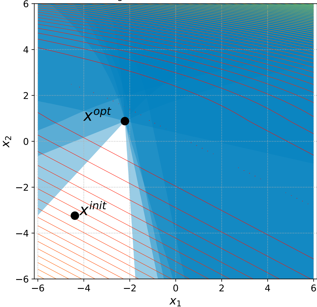
33 Bent Cigar with 6 constraints, instance=15
