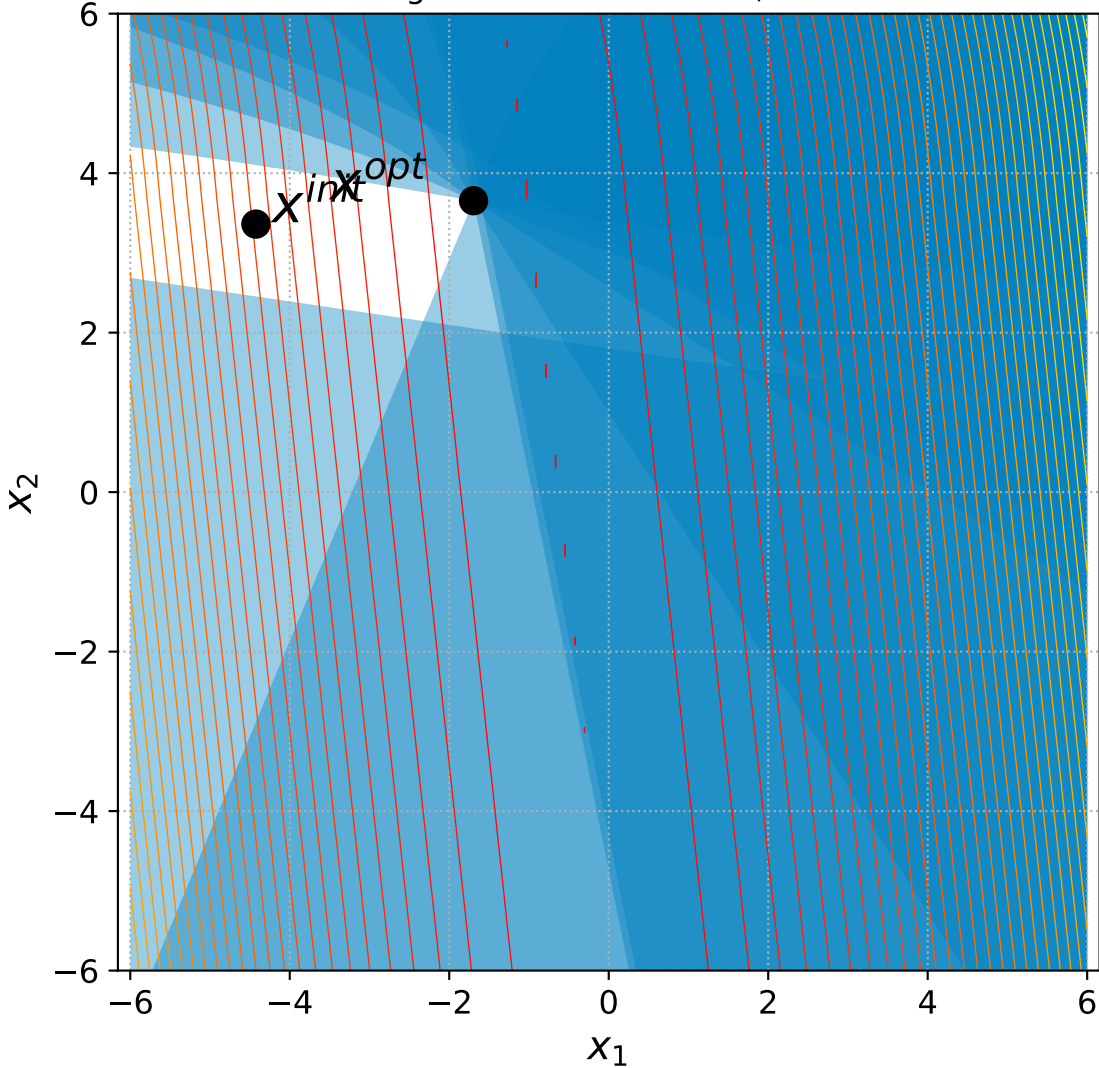
33 Bent Cigar with 6 constraints, instance=14
