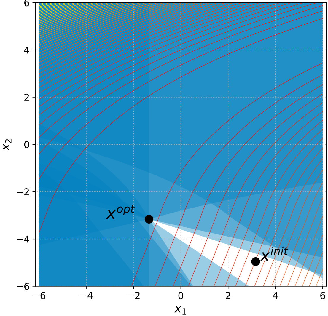
33 Bent Cigar with 6 constraints, instance=11
