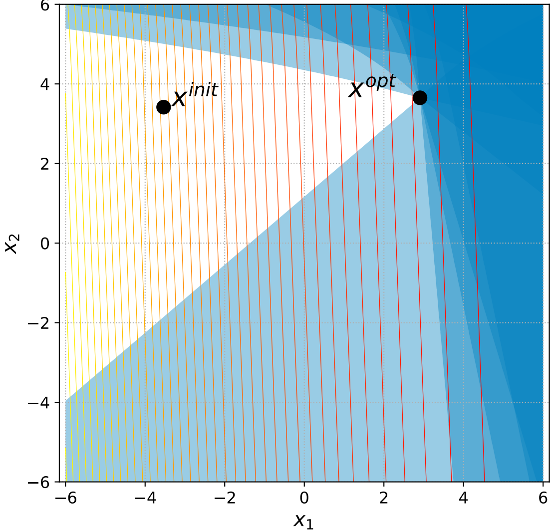
33 Bent Cigar with 6 constraints, instance=10
