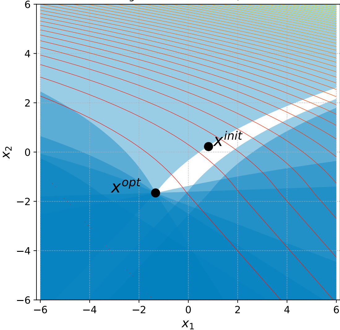
33 Bent Cigar with 6 constraints, instance=9
