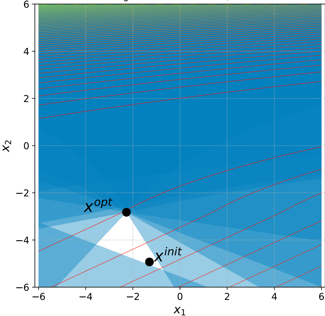
33 Bent Cigar with 6 constraints, instance=4
