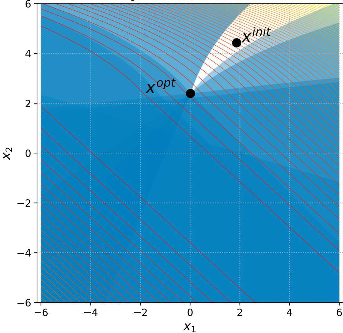
33 Bent Cigar with 6 constraints, instance=3
