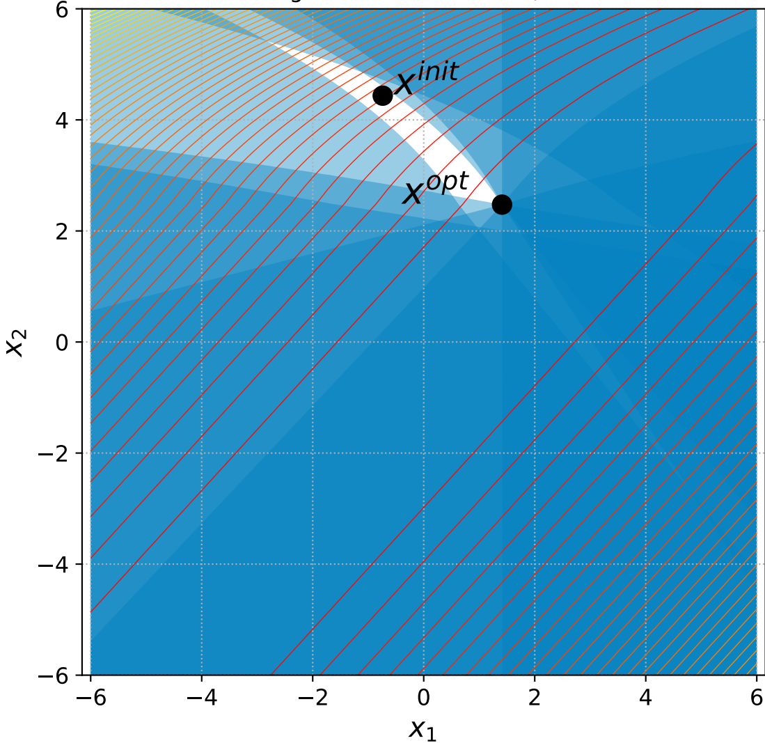
33 Bent Cigar with 6 constraints, instance=1
