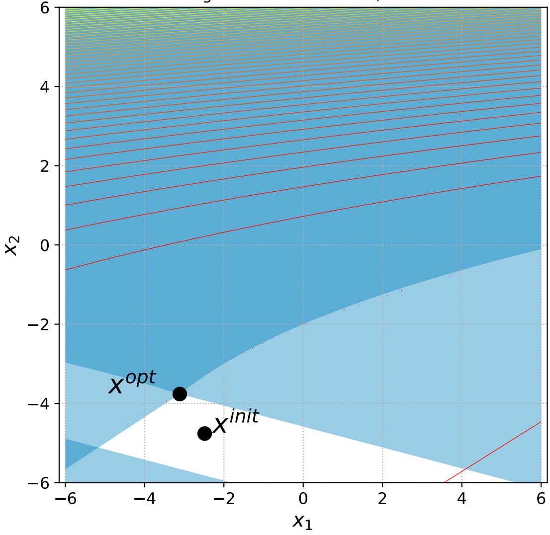
32 Bent Cigar with 2 constraints, instance=15
