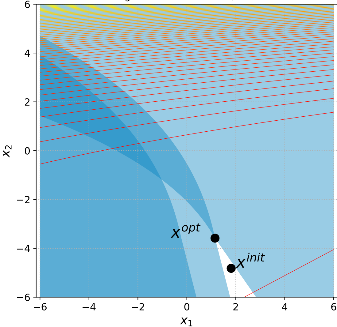
32 Bent Cigar with 2 constraints, instance=14
