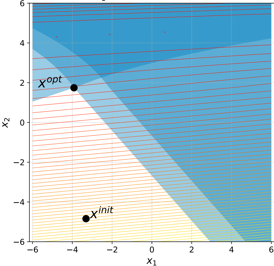
32 Bent Cigar with 2 constraints, instance=13
