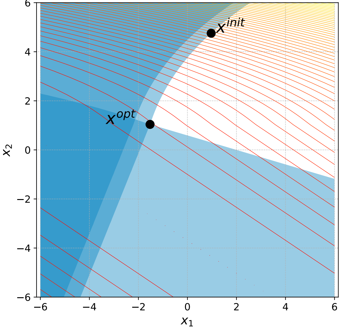
32 Bent Cigar with 2 constraints, instance=12
