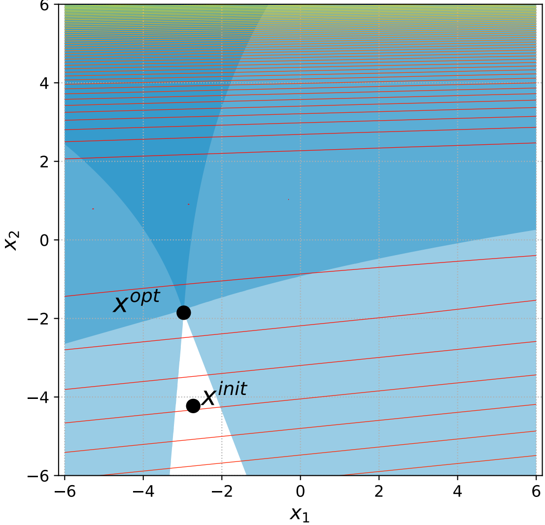
32 Bent Cigar with 2 constraints, instance=11
