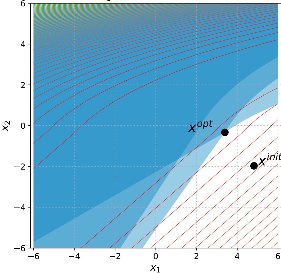
32 Bent Cigar with 2 constraints, instance=9
