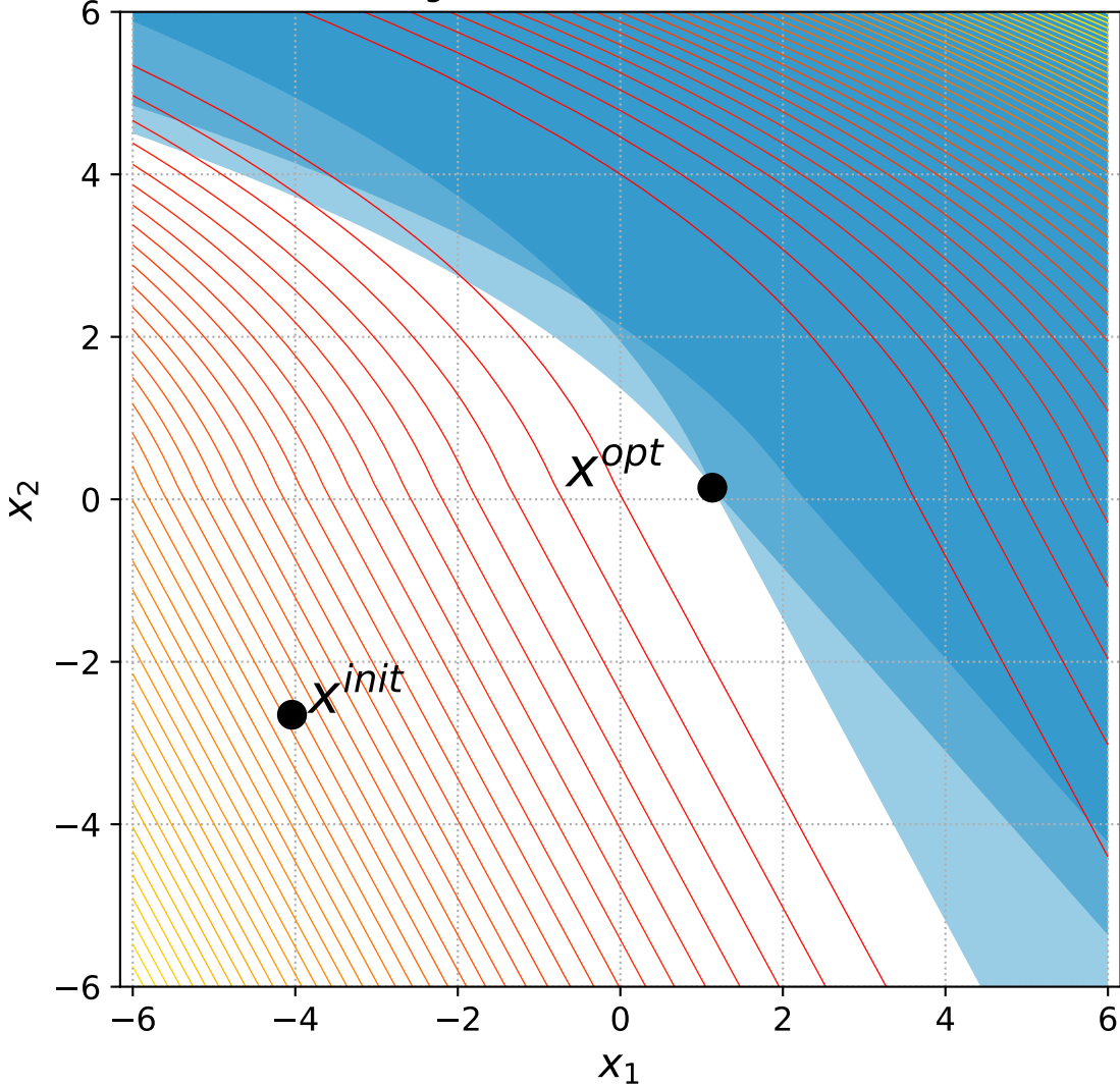
32 Bent Cigar with 2 constraints, instance=8
