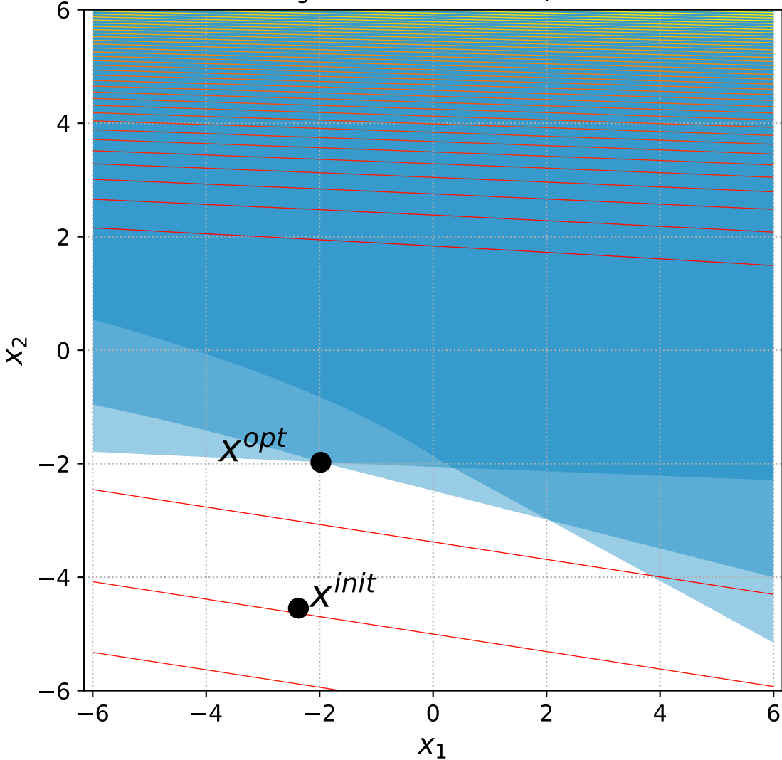
32 Bent Cigar with 2 constraints, instance=7
