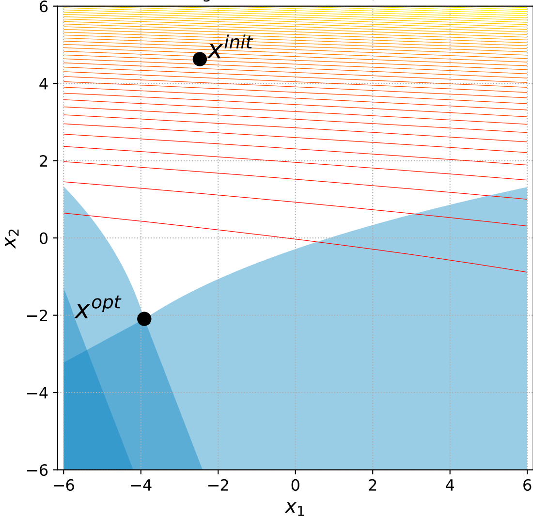
32 Bent Cigar with 2 constraints, instance=6
