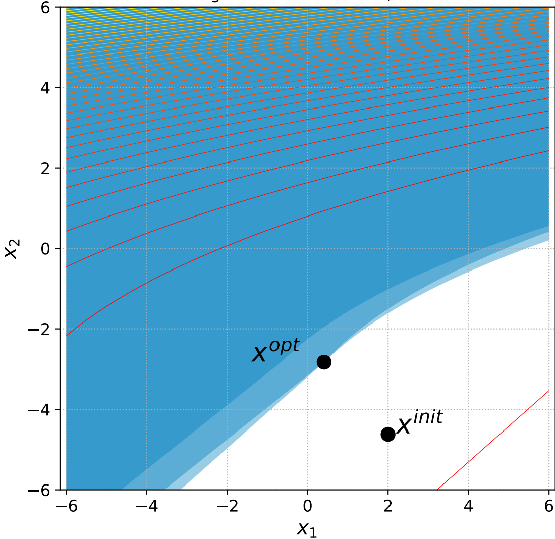
32 Bent Cigar with 2 constraints, instance=3
