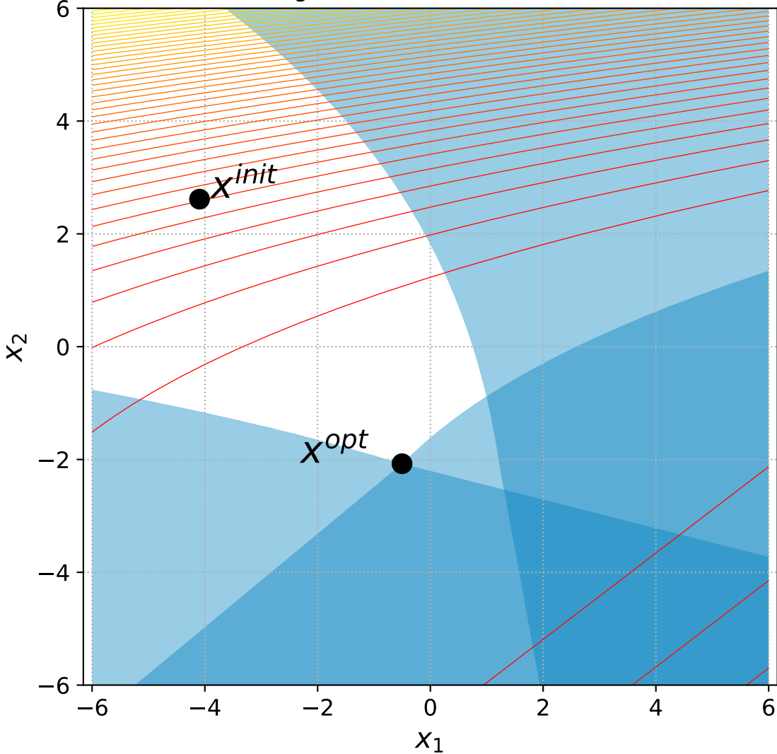
32 Bent Cigar with 2 constraints, instance=2
