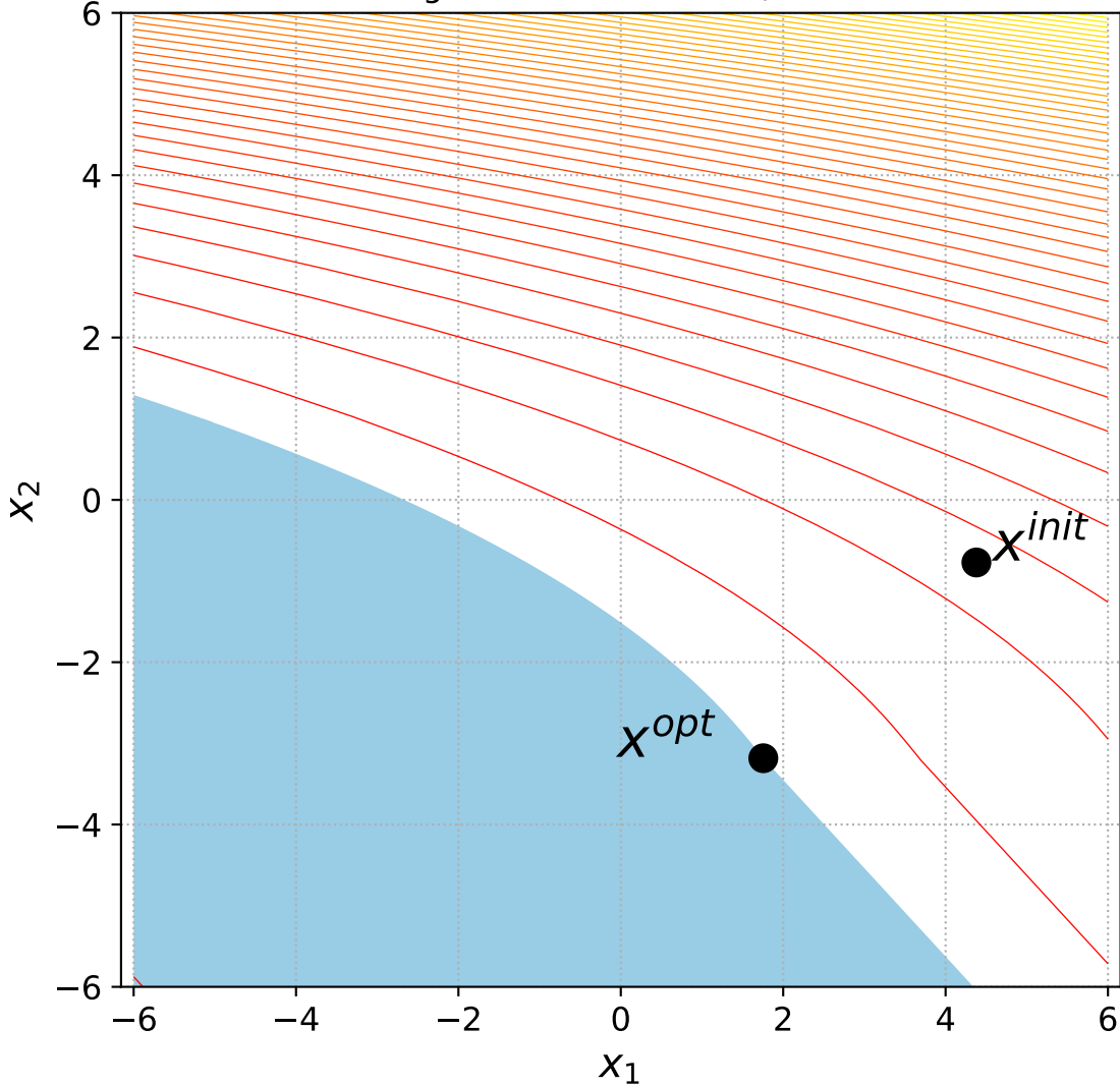
31 Bent Cigar with 1 constraint, instance=14
