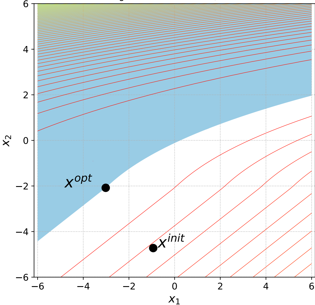
31 Bent Cigar with 1 constraint, instance=12
