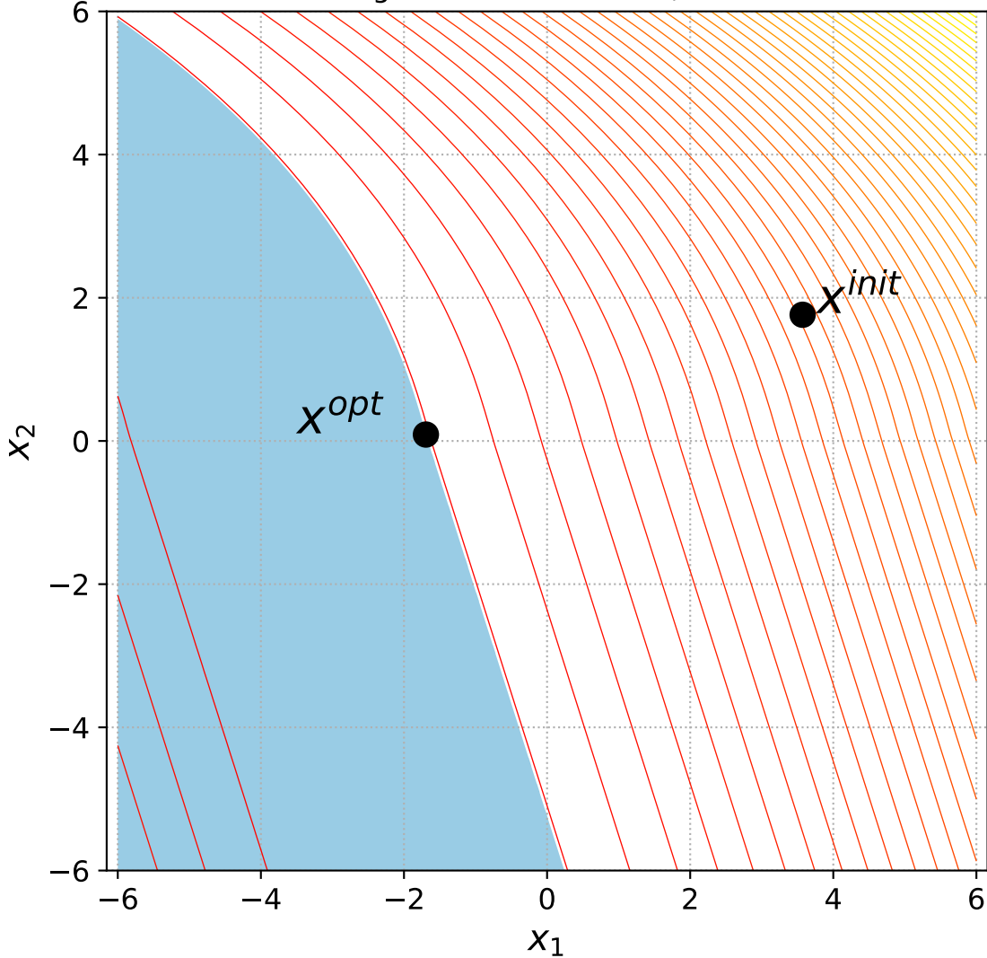
31 Bent Cigar with 1 constraint, instance=11
