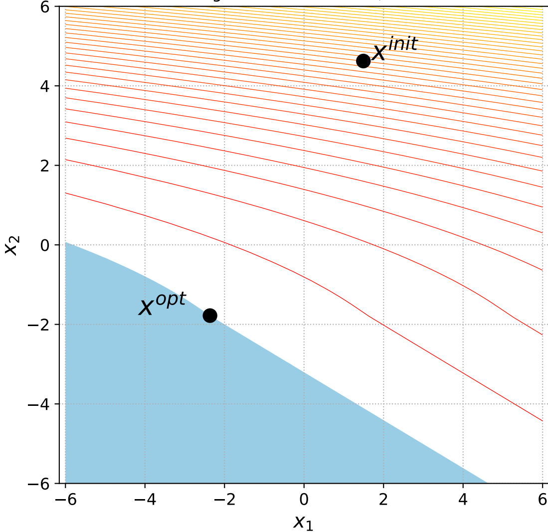
31 Bent Cigar with 1 constraint, instance=9
