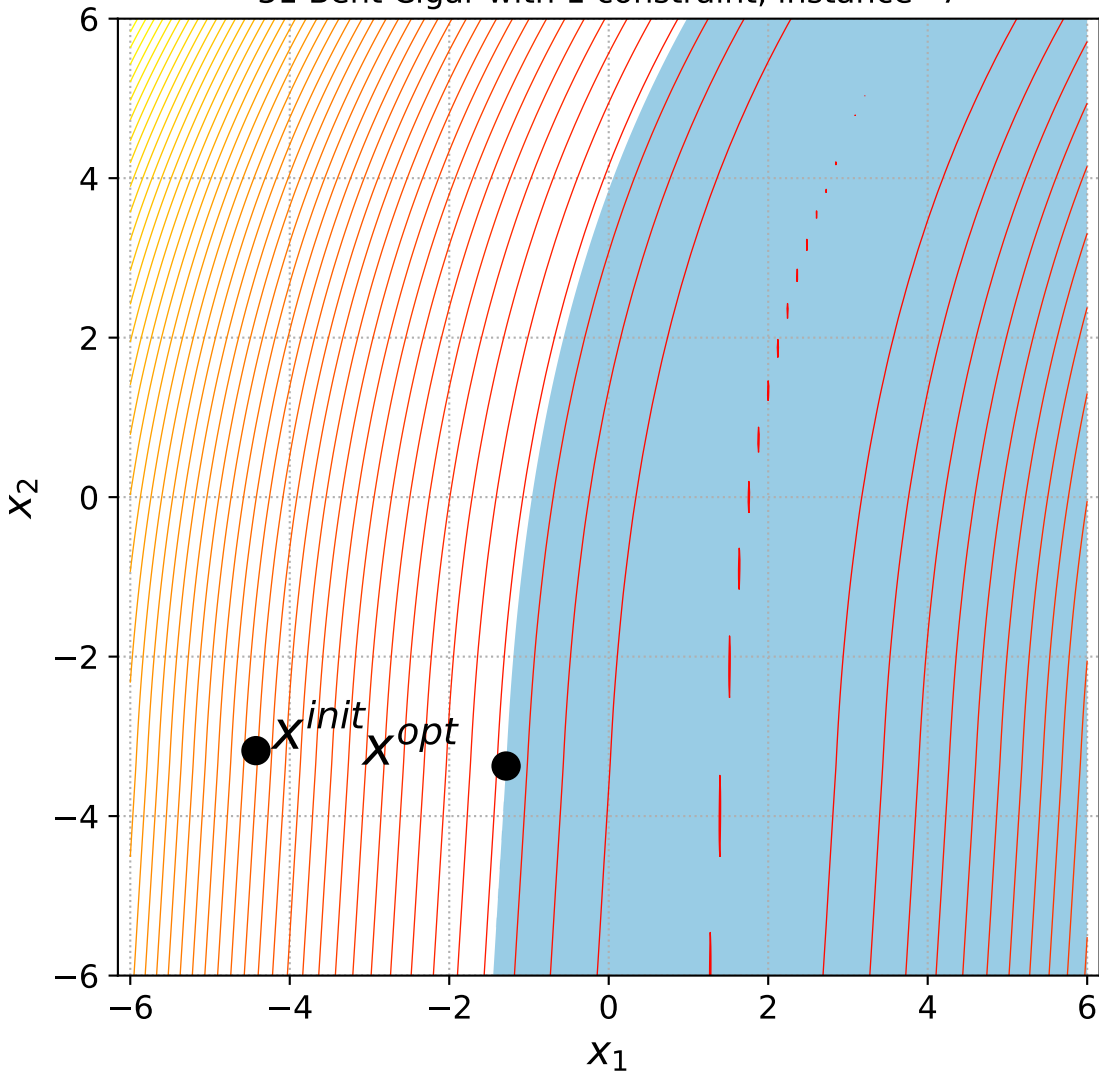
31 Bent Cigar with 1 constraint, instance=7
