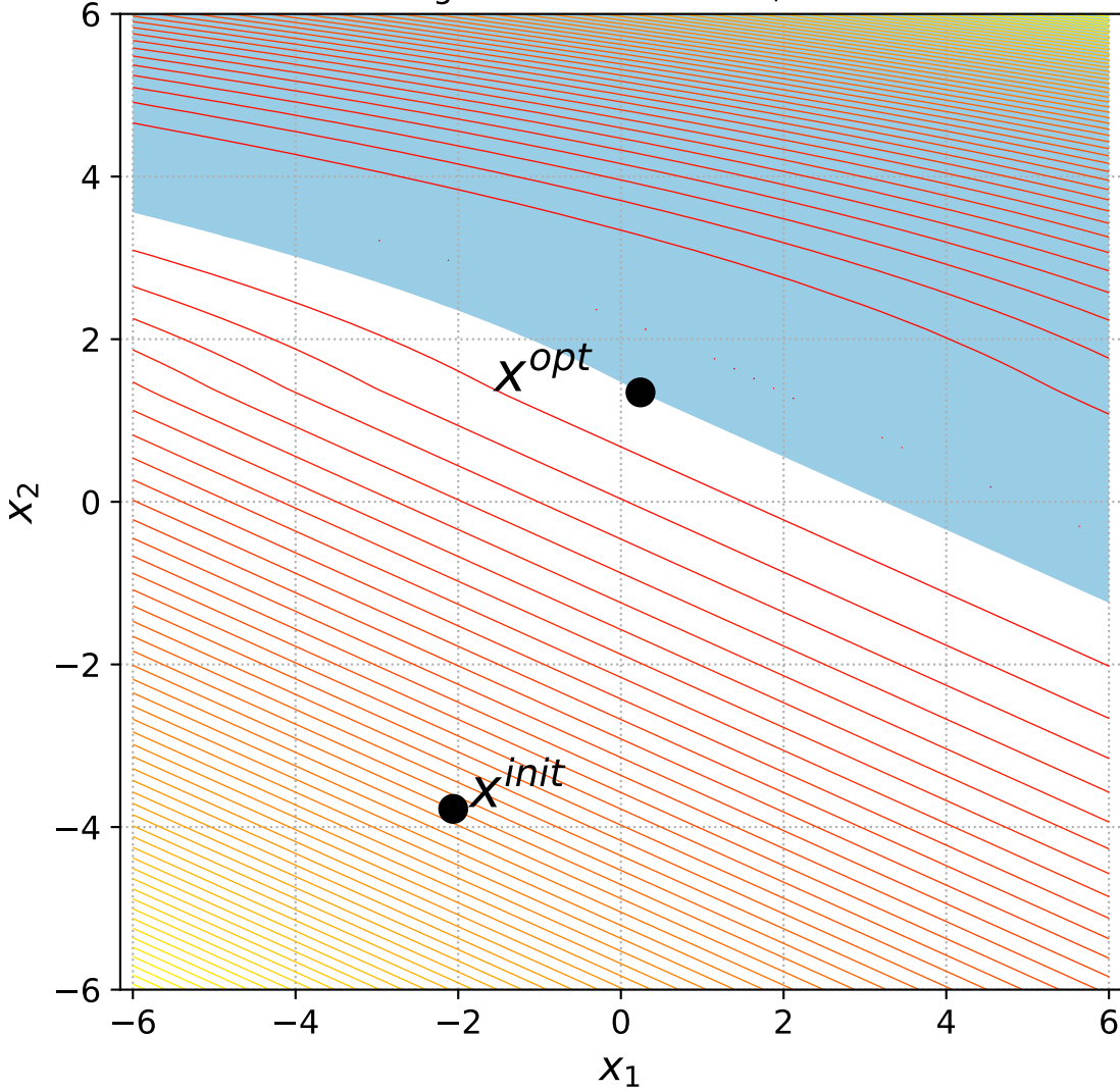
31 Bent Cigar with 1 constraint, instance=5
