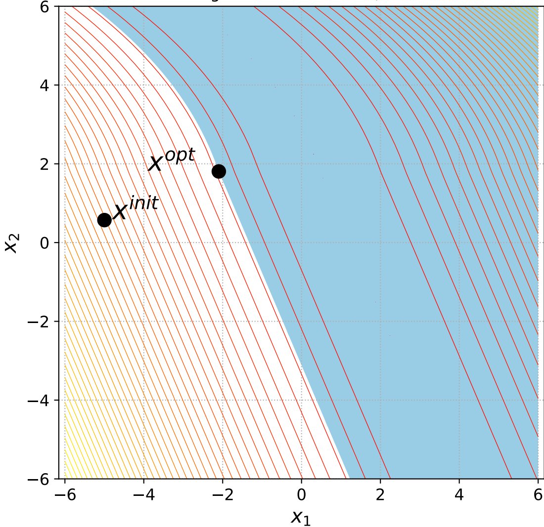
31 Bent Cigar with 1 constraint, instance=3
