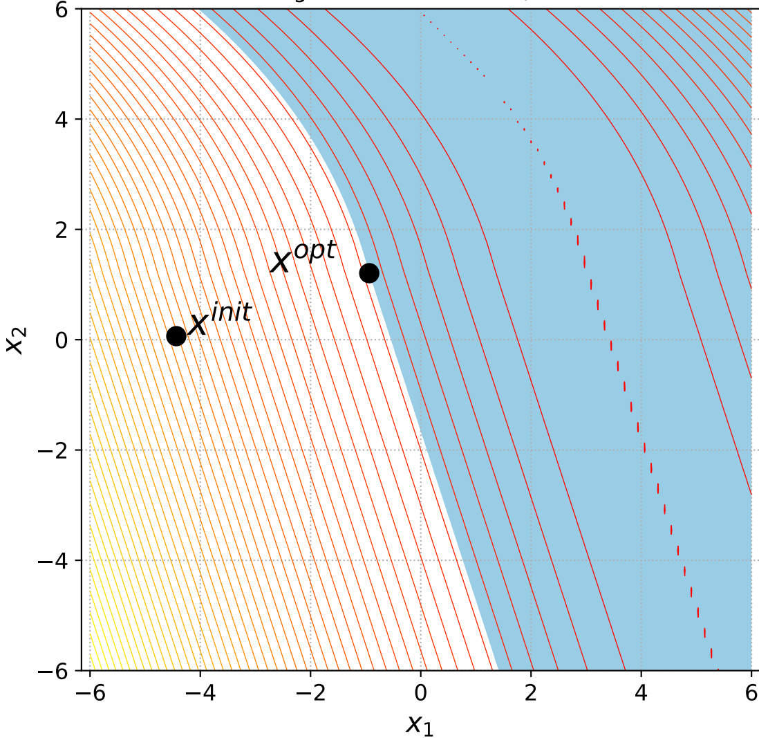
31 Bent Cigar with 1 constraint, instance=2
