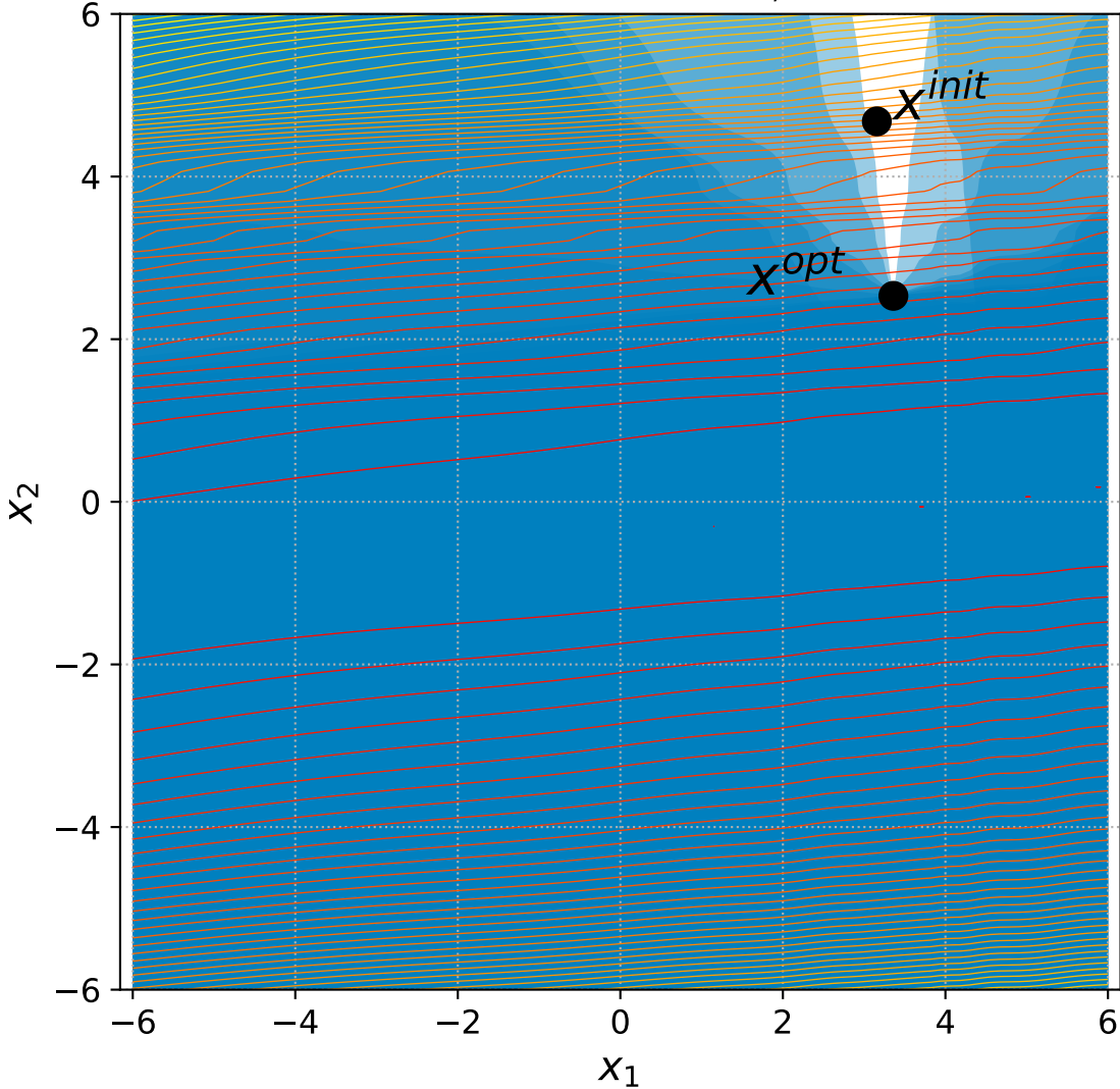
30 Discus with 6+3n constraints, instance=15
