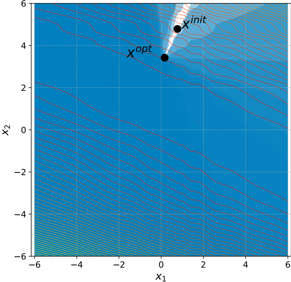
30 Discus with 6+3n constraints, instance=11
