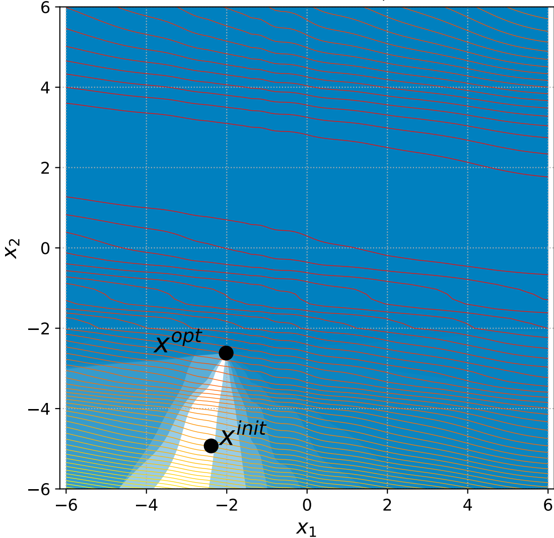
30 Discus with 6+3n constraints, instance=10
