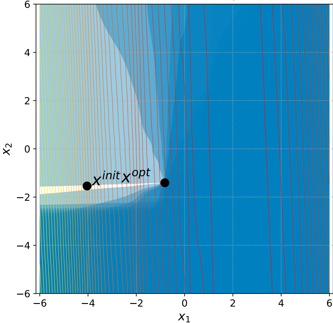
30 Discus with 6+3n constraints, instance=9
