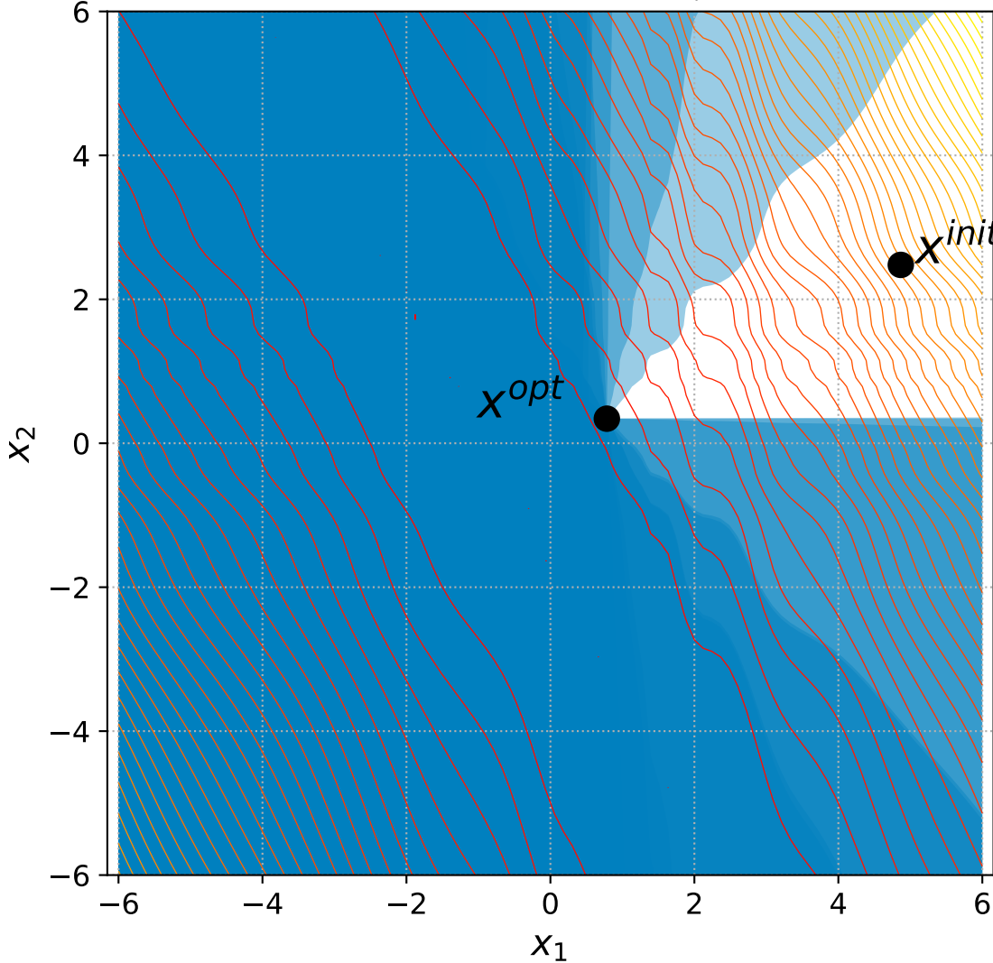
30 Discs with 6+3n constraints, instance=7
