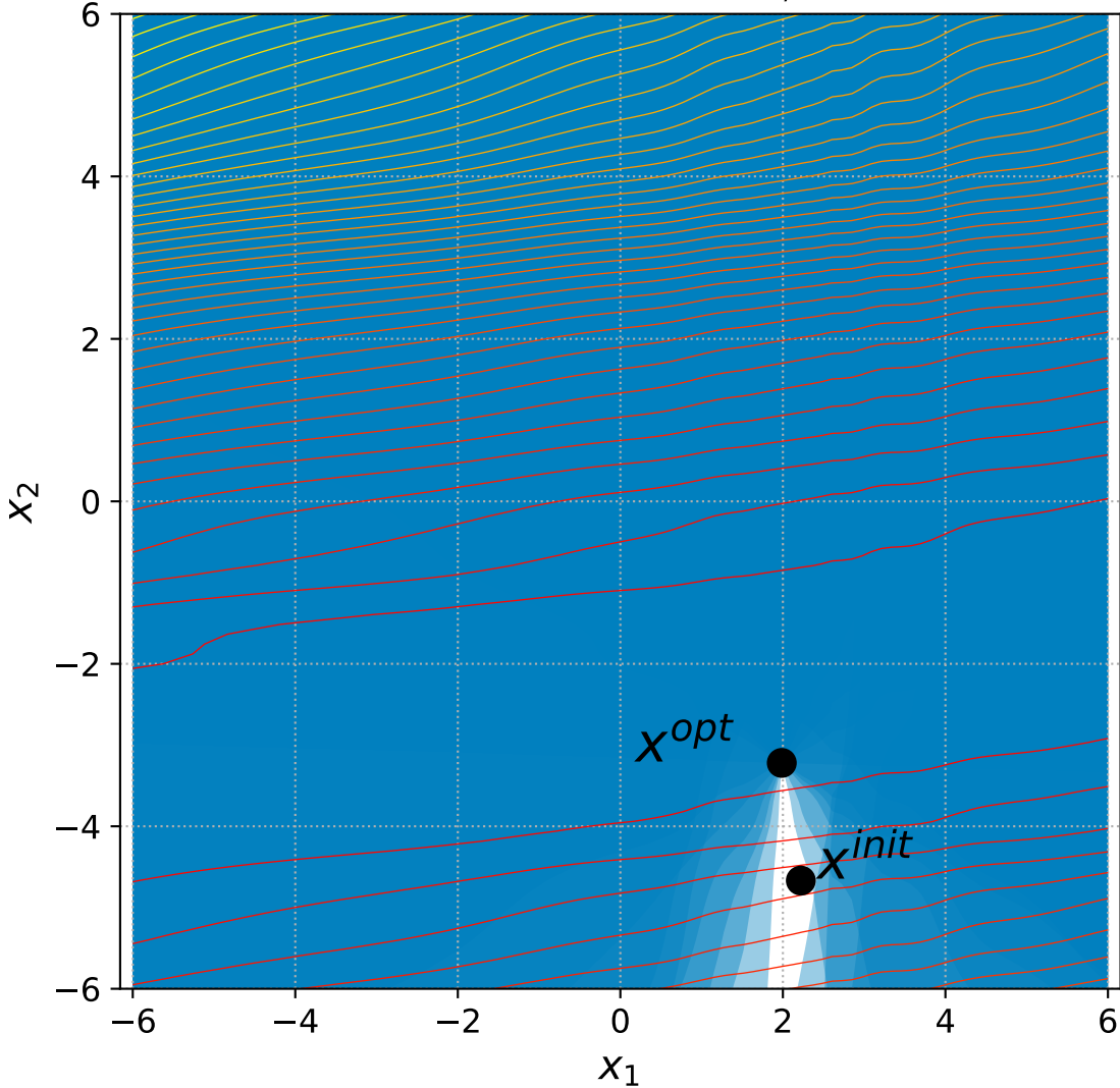
30 Discus with 6+3n constraints, instance=6
