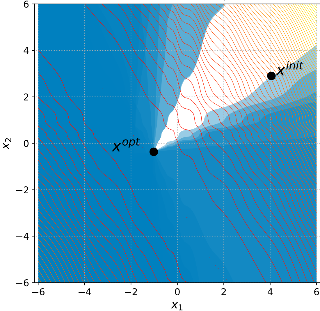
30 Discus with 6+3n constraints, instance=4
