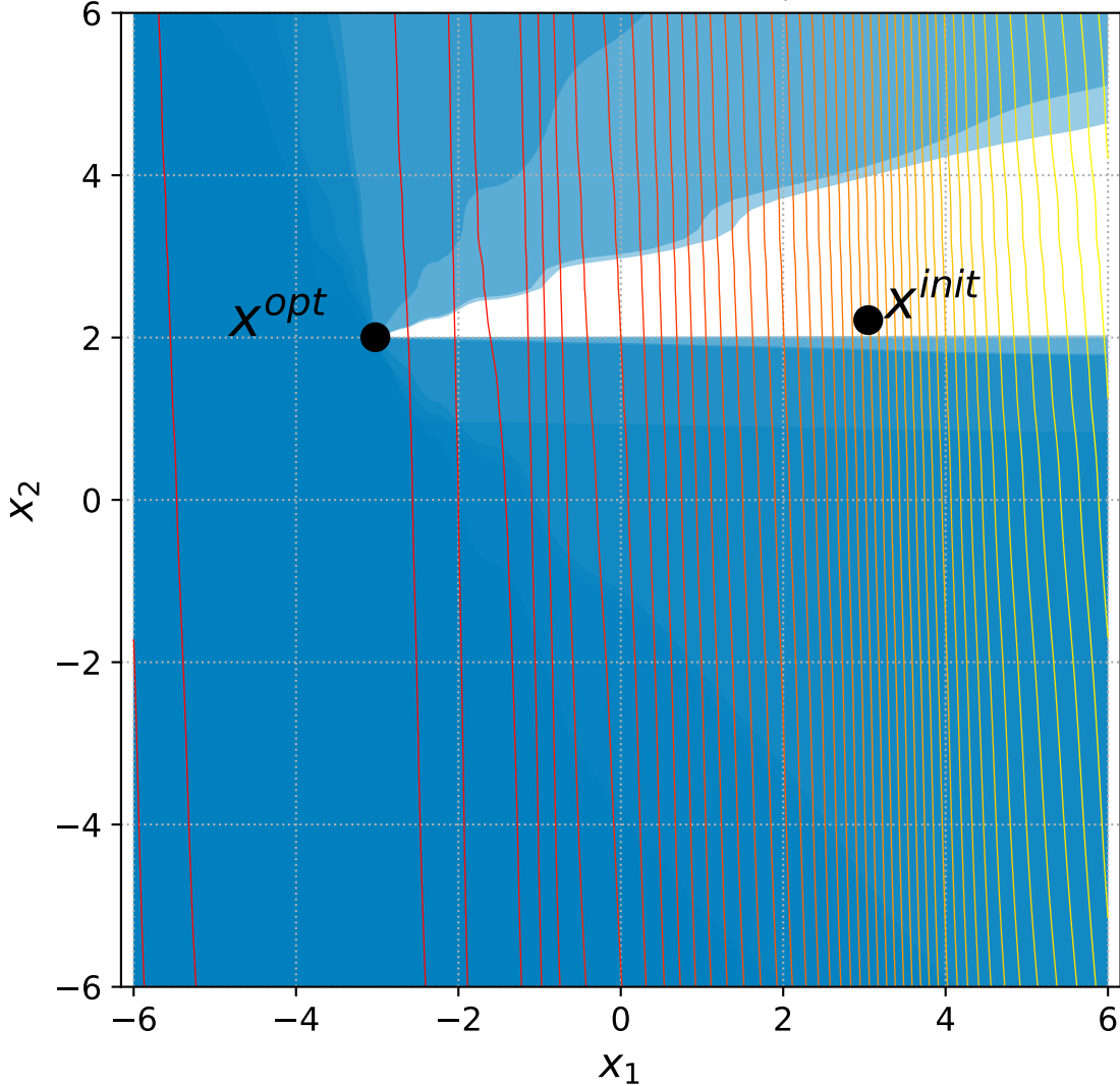
30 Discus with 6+3n constraints, instance=2
