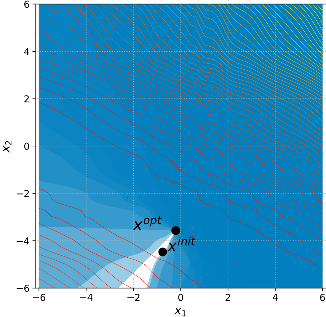
30 Discus with 6+3n constraints, instance=1
