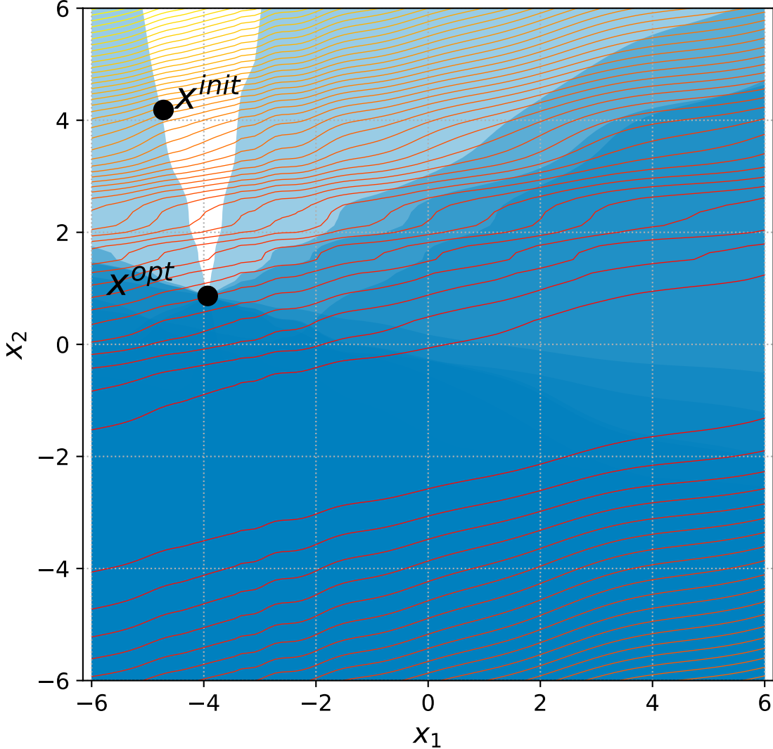
29 Discus with 6+n constraints, instance=14
