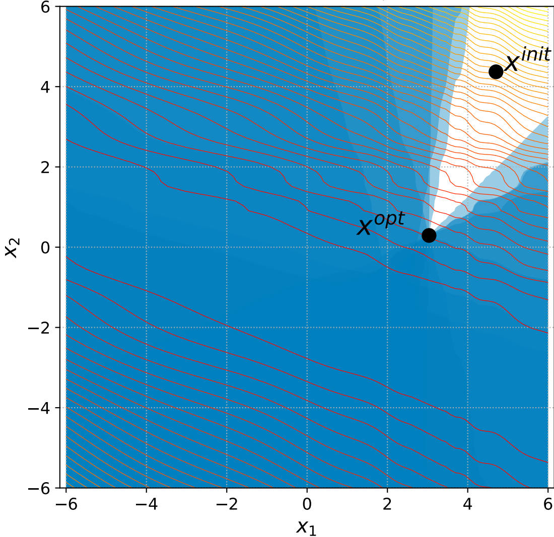
29 Discus with 6+n constraints, instance=9
