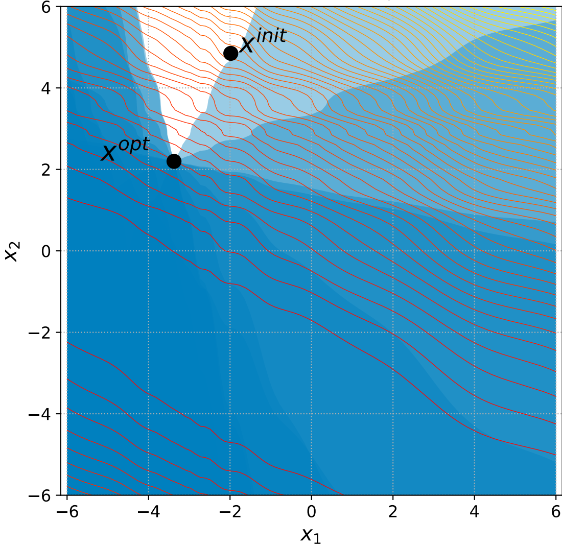
29 Discus with 6+n constraints, instance=8
