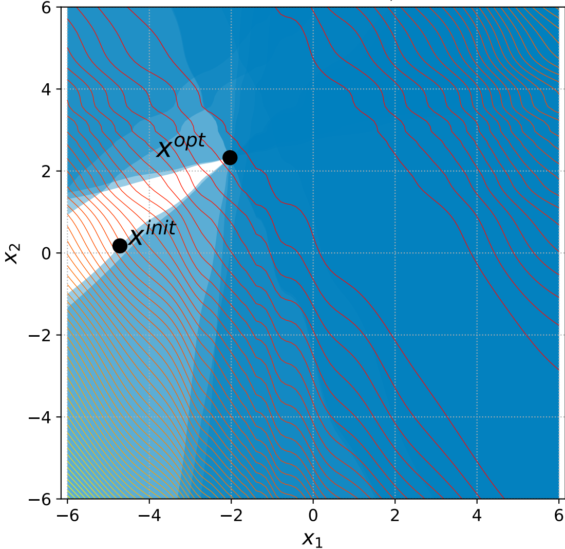
29 Discus with 6+n constraints, instance=6
