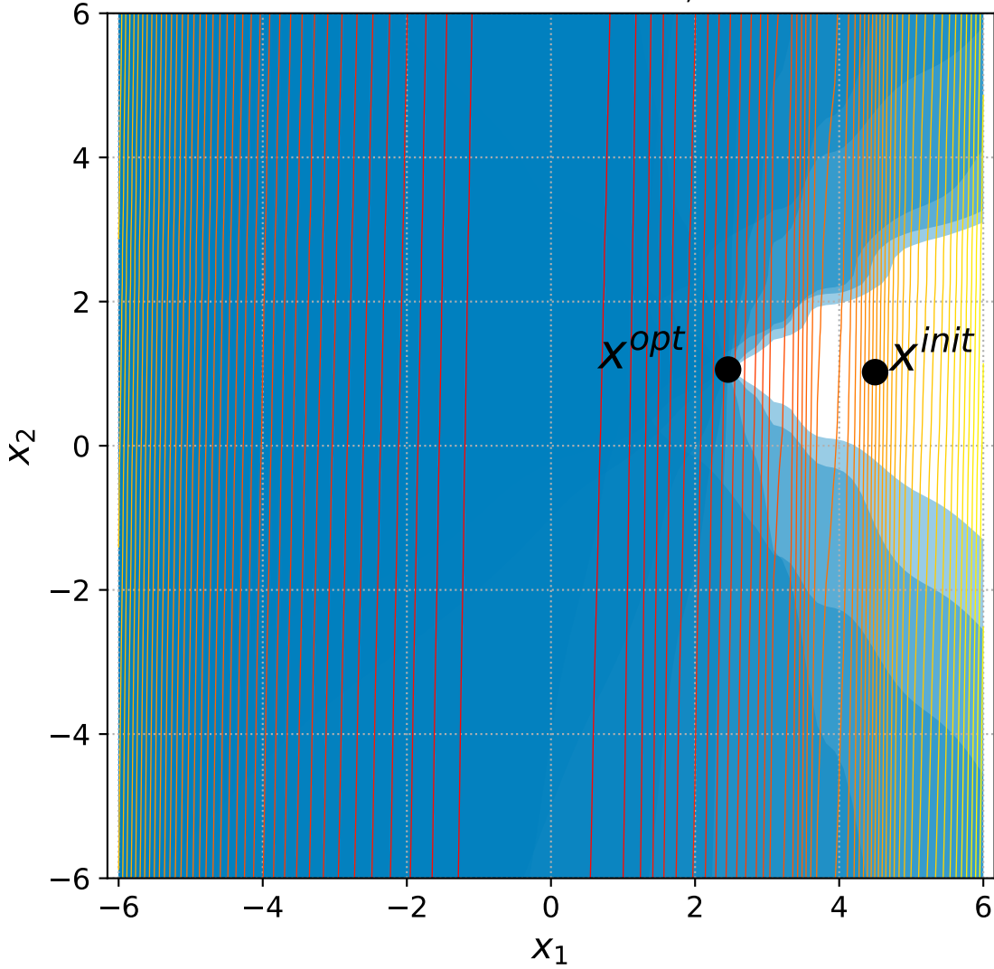
29 Discus with 6+n constraints, instance=5
