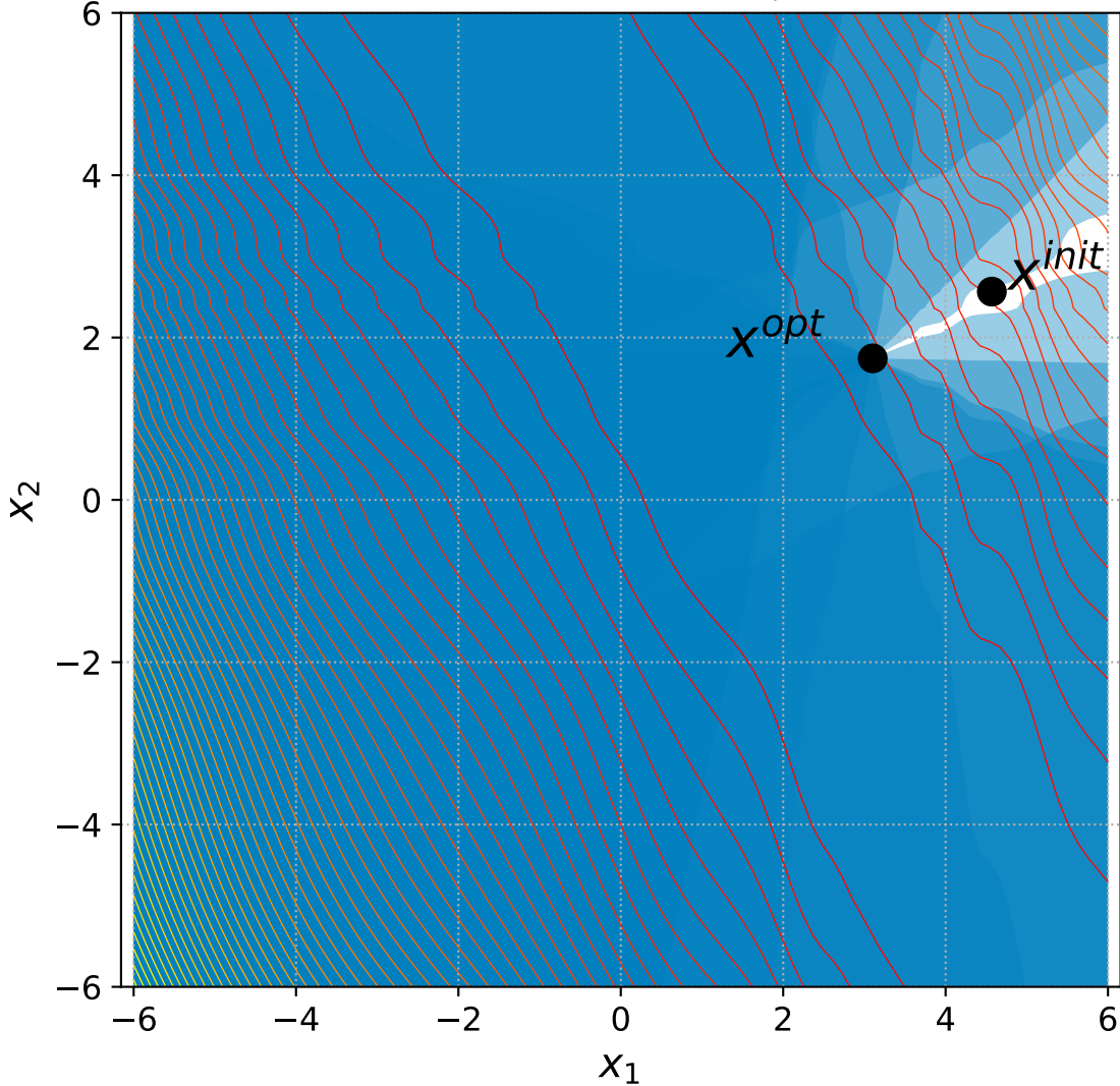
29 Discus with 6+n constraints, instance=4
