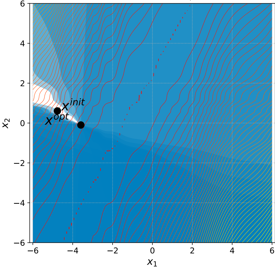
29 Discus with 6+n constraints, instance=2
