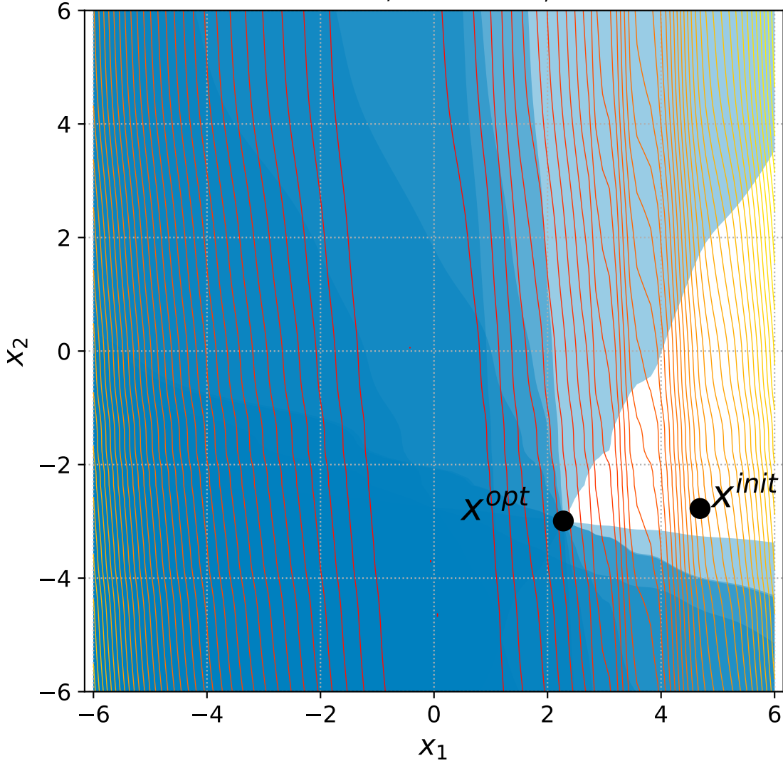
28 Discus with 6+n/2 constraints, instance=14
