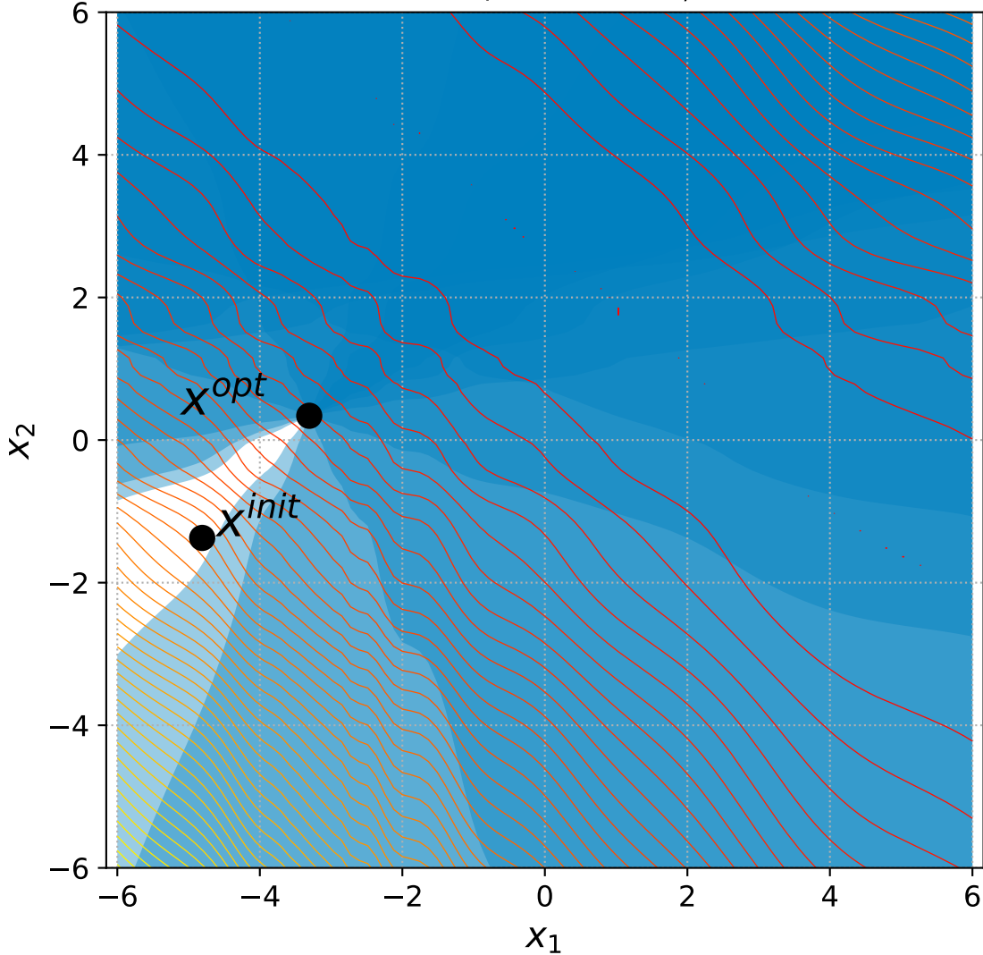
28 Discus with 6+n/2 constraints, instance=13
