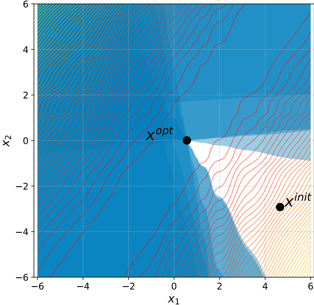
28 Discus with 6+n/2 constraints, instance=10
