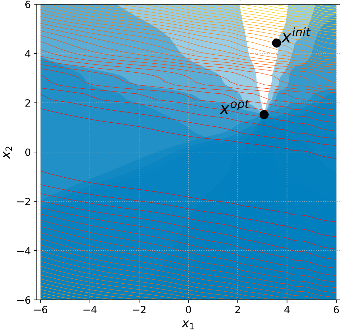
28 Discus with 6+n/2 constraints, instance=7
